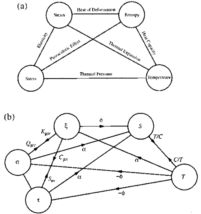
FIG. 1. Schematic diagram showing the relations between various thermodynamic variables. (a) The names of the properties and the variables. (b) The corresponding symbols.
